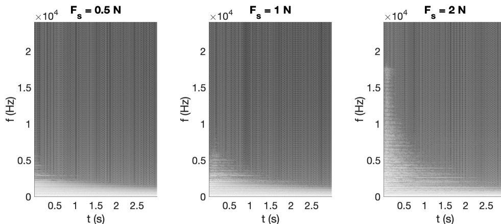
Figure 7: Displacement spectrograms for the three case studies. Input forcing amplitudes as indicated. The sample rate used is 48 kHz.
