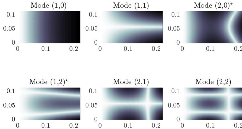
Fig. 3. Modal shapes for a plate with \sigma = 223/114 , B = \{C-F-F-F\} , p = 6.53, q = 0.29 . Modes (1,2) and (2,0) are marked with a star as assigning unambiguous modal indices may be difficult in some cases. See also Fig. 2.
